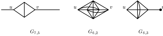
Figure 1: Examples of graphs G_{n,d} .
